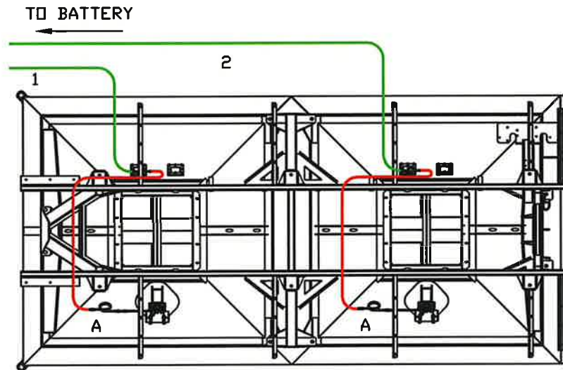
VIEW FROM BOTTOM OF THE BOX LOOKING UP
