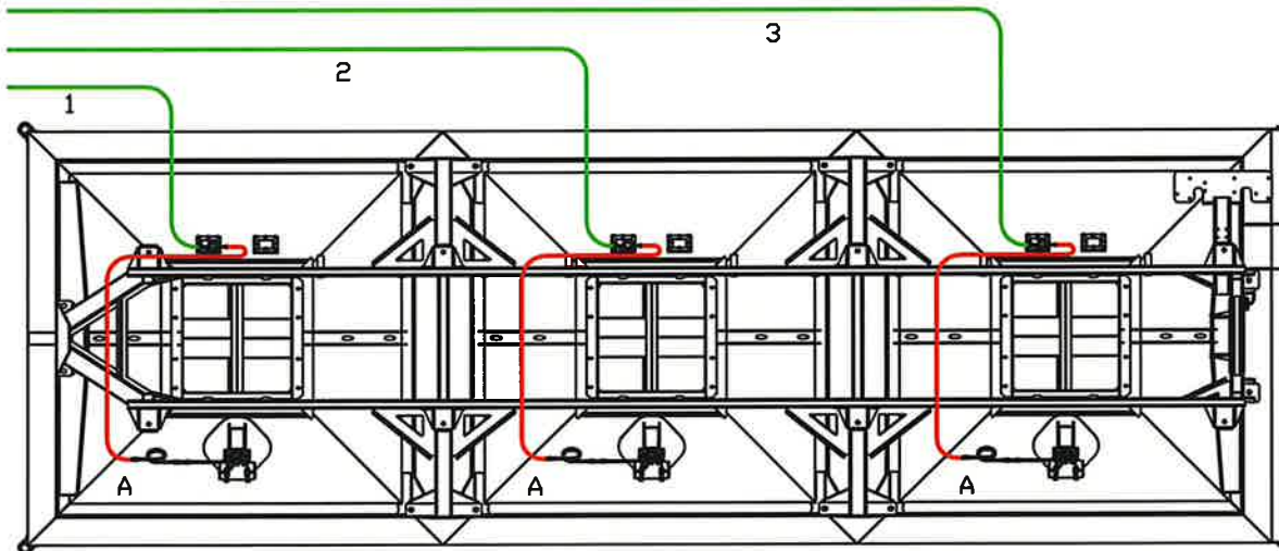
VIEW FROM BOTTOM OF THE BOX LOOKING UP
